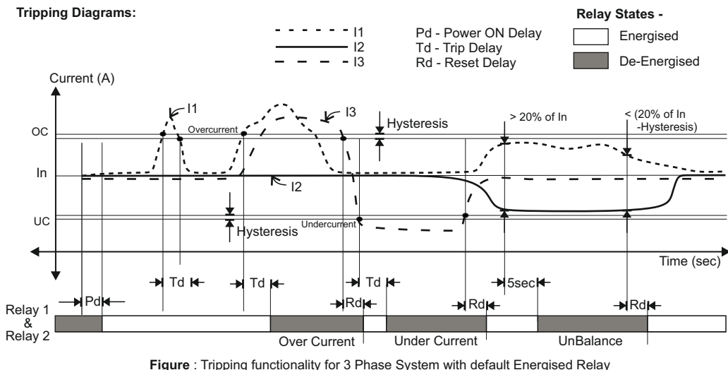
Figure : Tripping functionality for 3 Phase System with default Energised Relay
